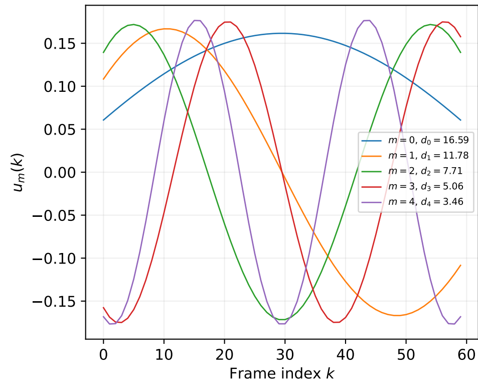
Eigenvectors of \Sigma_0 (first 5)
