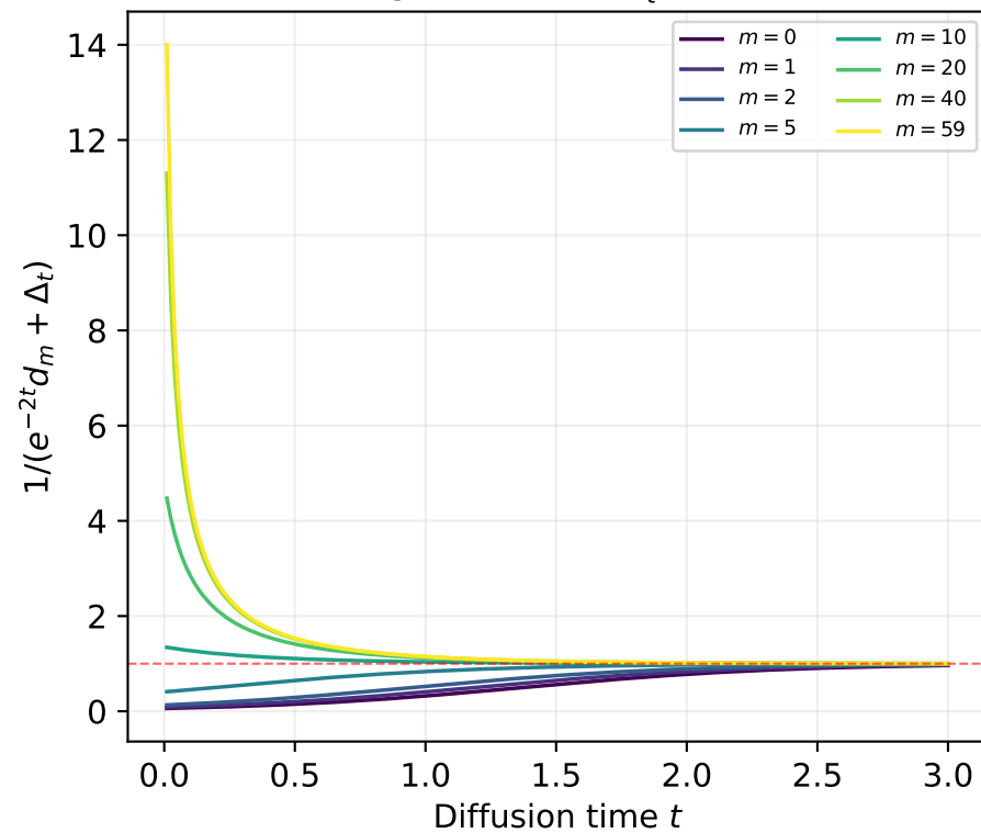
Eigenvalues of \Sigma_t^{-1} vs t
