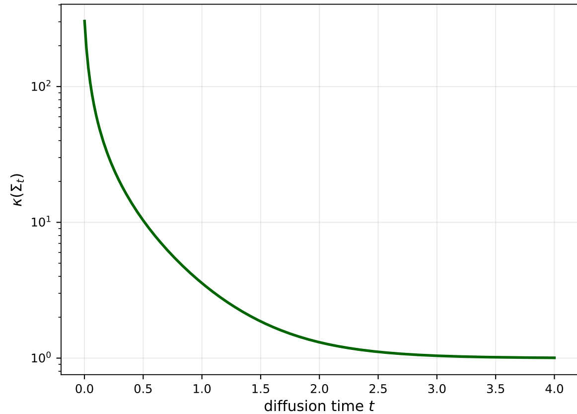
Condition number of \Sigma_t
