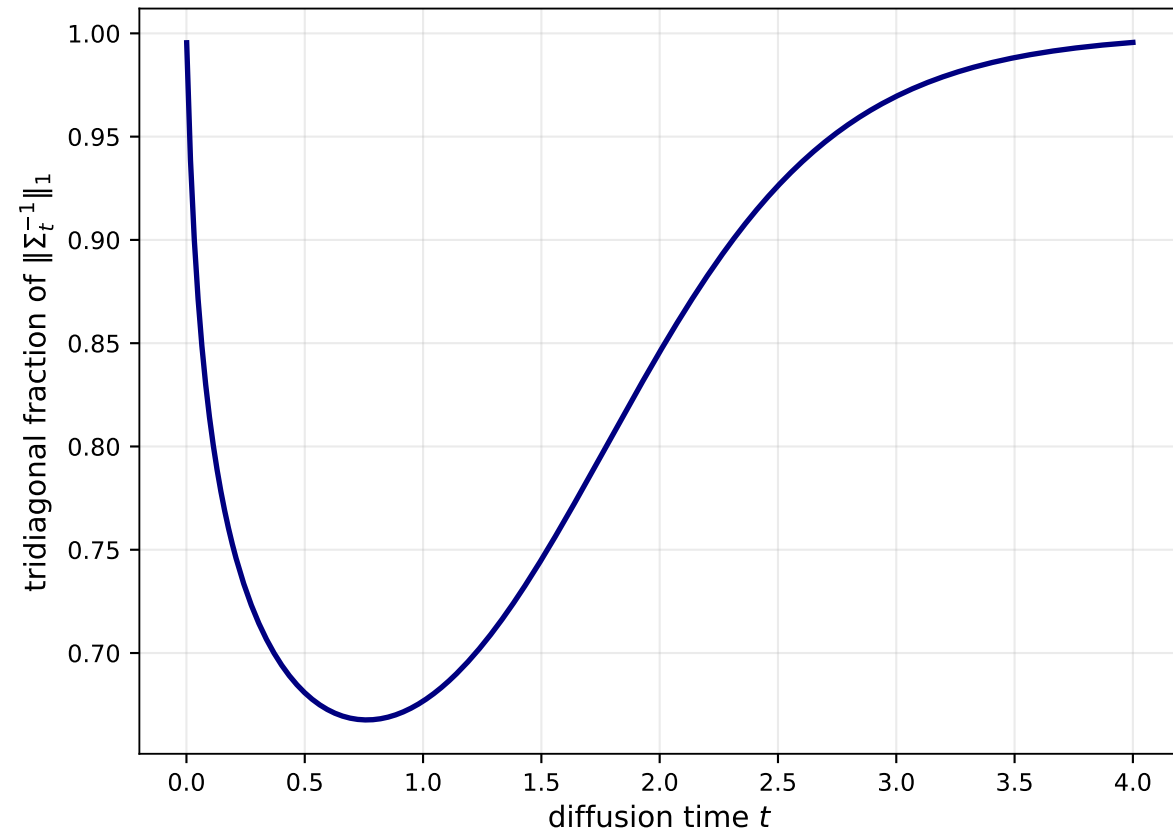
Loss of tridiagonal concentration
