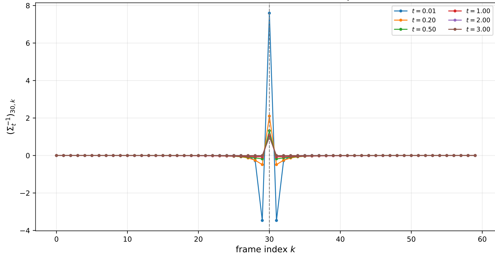
Coupling profile of a central row of \Sigma_t^{-1}
