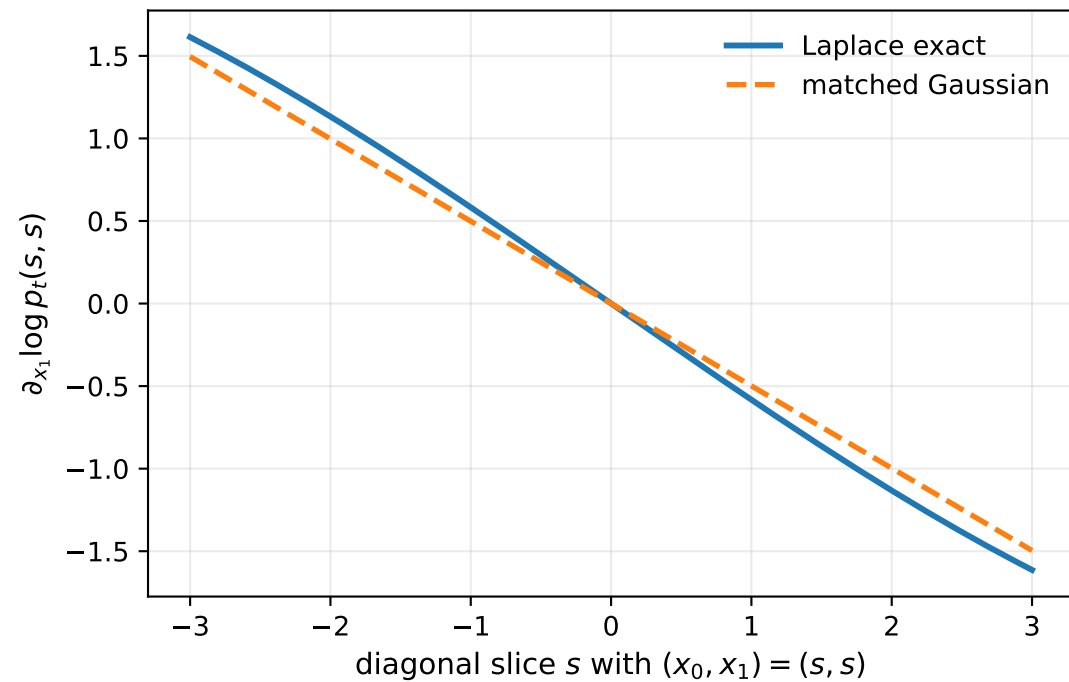
Second-coordinate score
