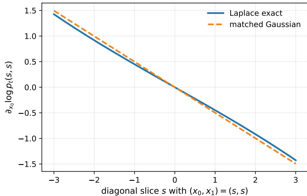
First-coordinate score
