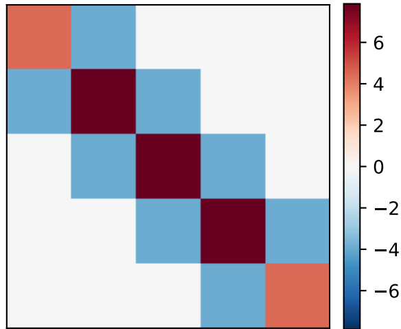
Q_t, t = 0.00
