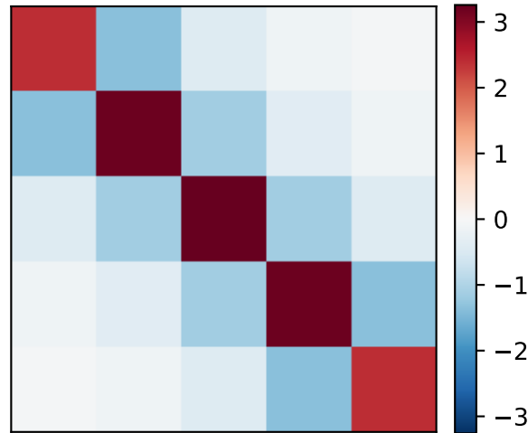
Q_t, t = 0.08
