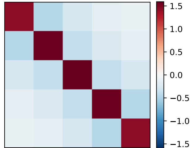
Q_t, t = 0.30
