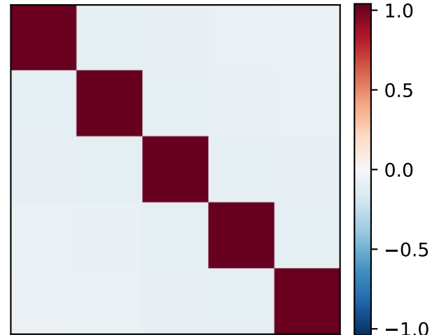
Q_t, t = 1.00
