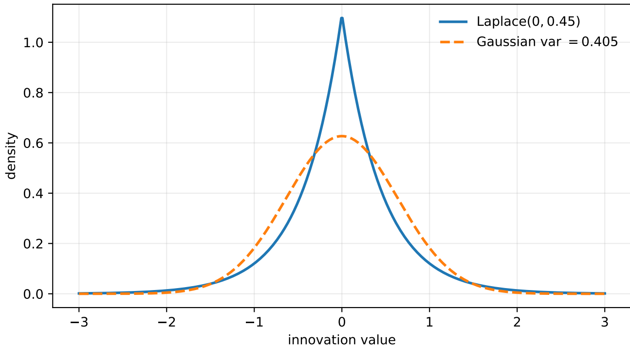
Matched-variance innovations: Laplace is sharper and heavier-tailed
