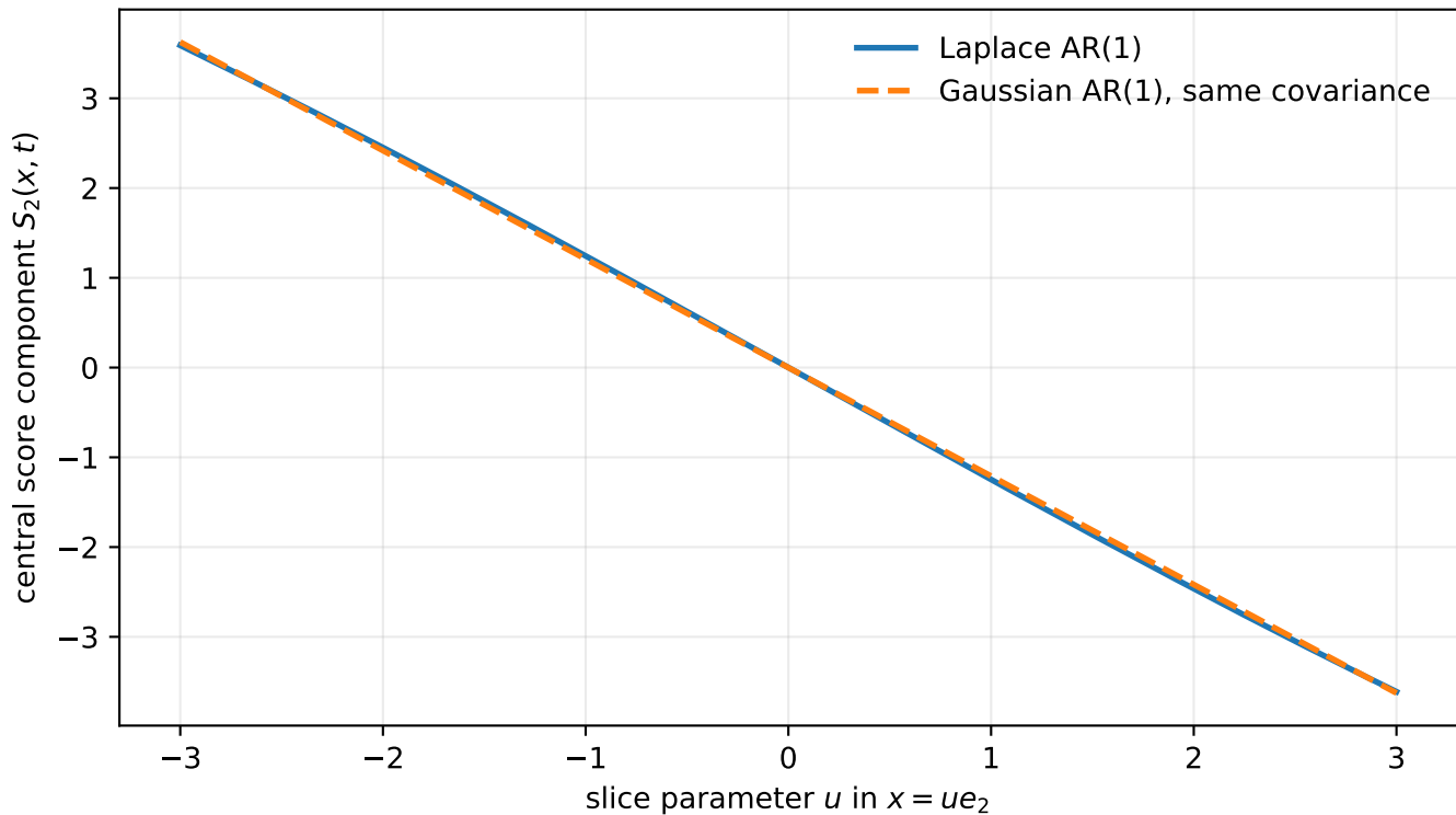
Non-Gaussian score is nonlinear; Gaussian score is affine
