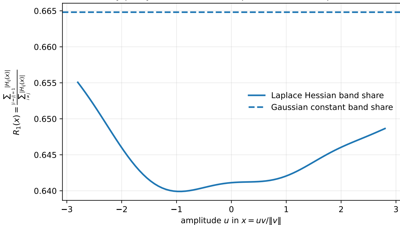
A locality proxy becomes state-dependent in the Laplace model
