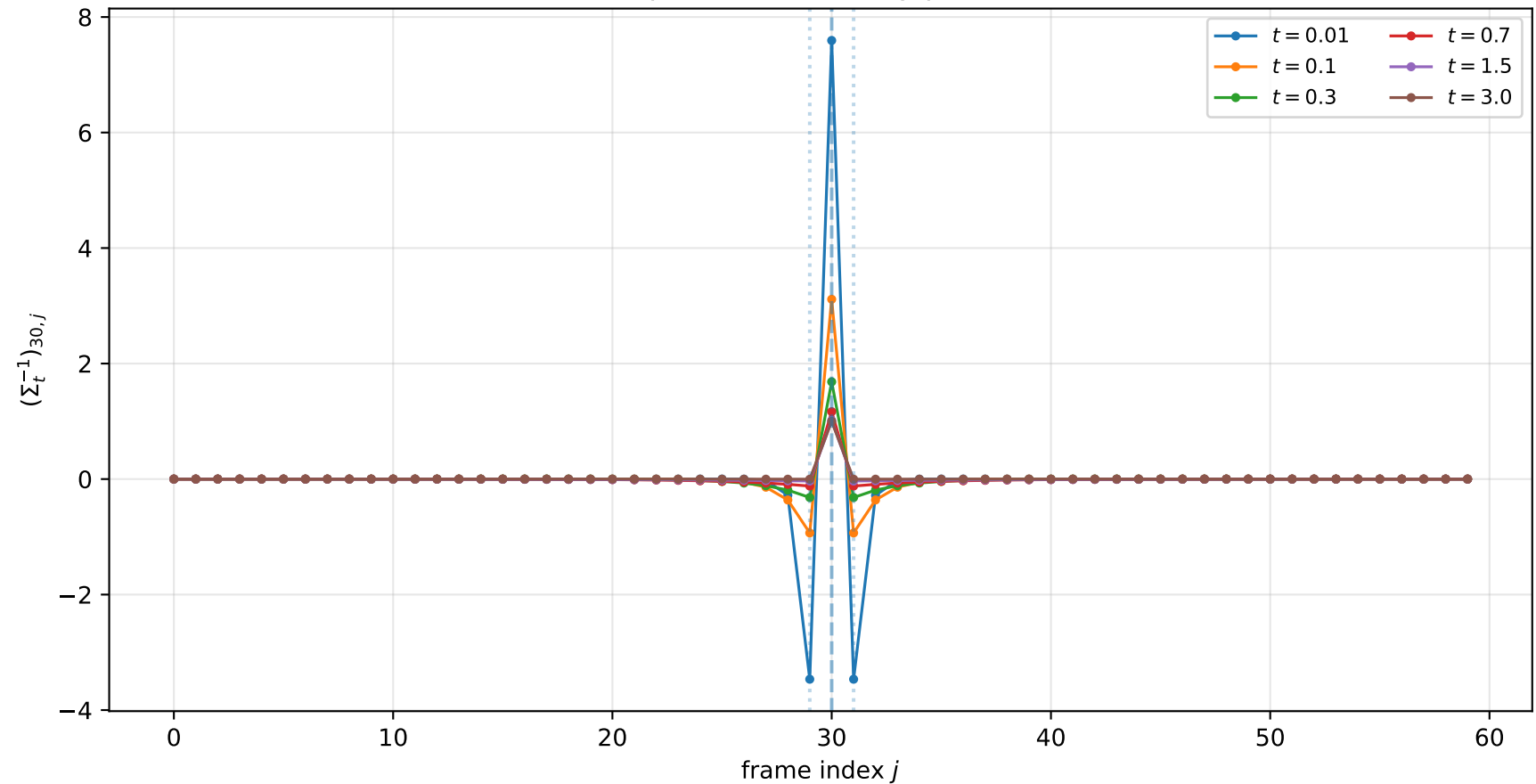
row profile of the noisy precision
