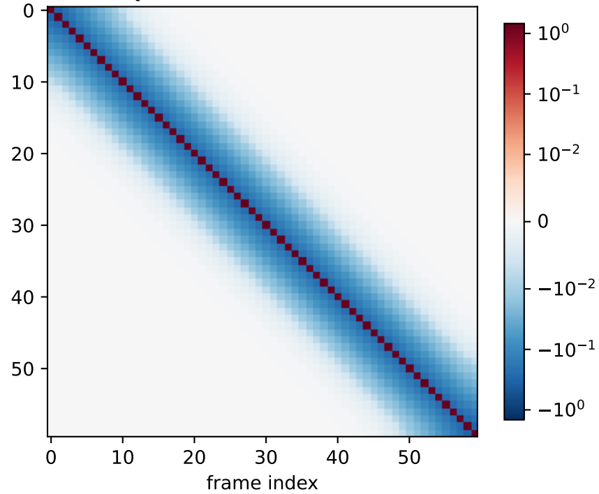
\Sigma_t^{-1} , symlog scale, t = 0.4
