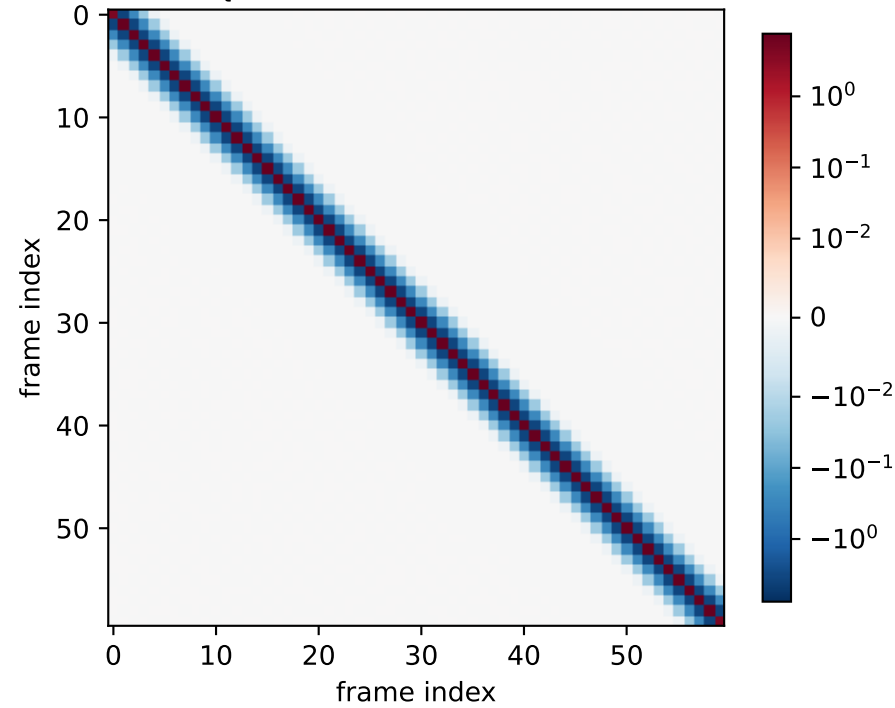
\Sigma_t^{-1} , symlog scale, t = 0.01
