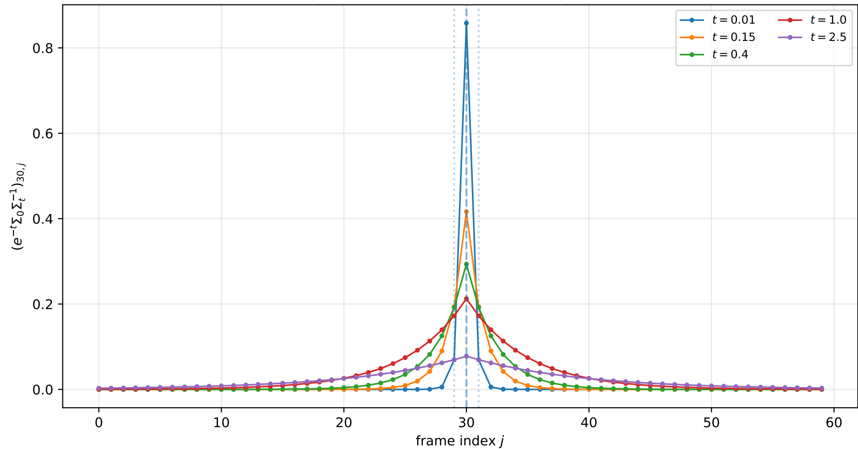
posterior-mean sensitivity row profile
