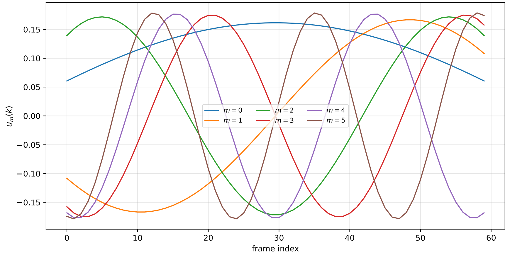
leading eigenvectors of \Sigma_0
