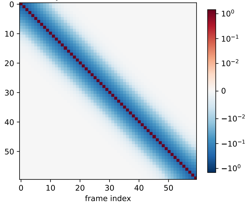
\Sigma_t^{-1} , symlog scale, t = 0.4
