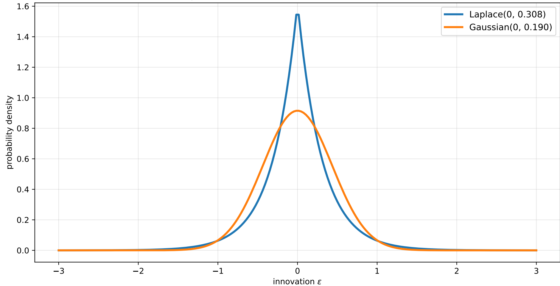
Laplace vs Gaussian innovations (same variance)
