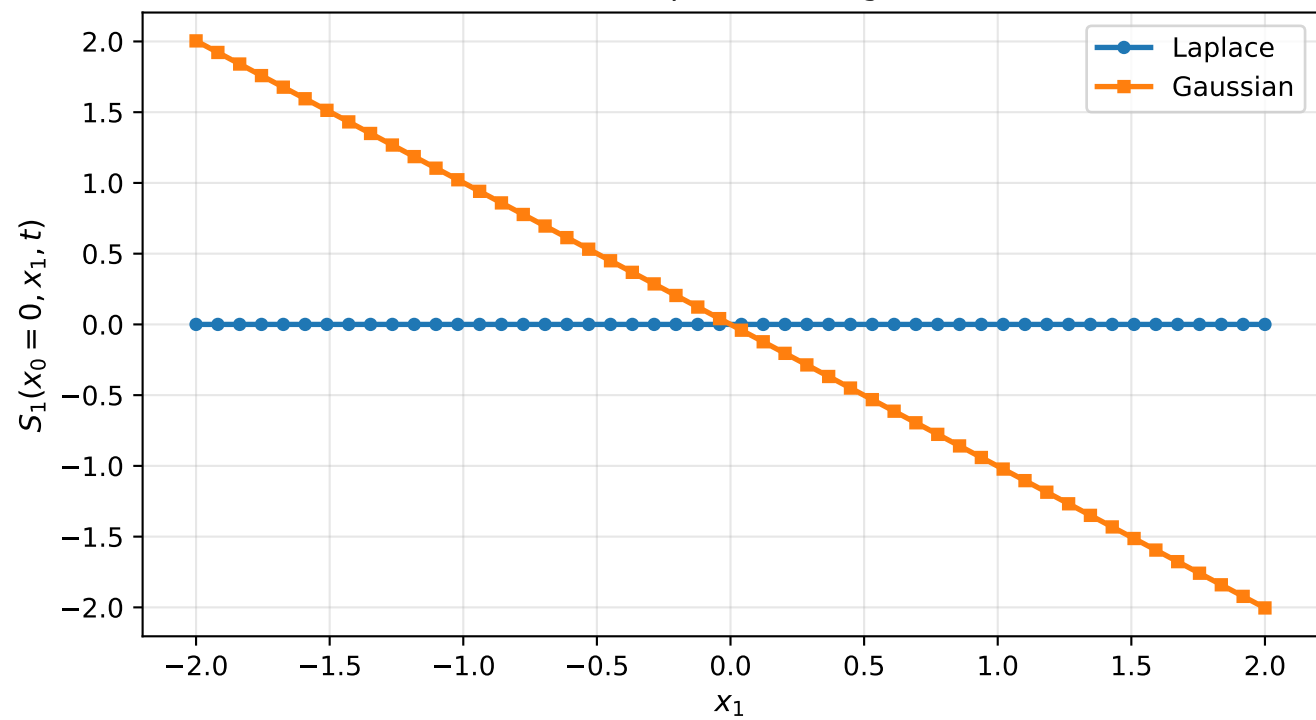
K=1: Score component along x_1 , t = 1.5
