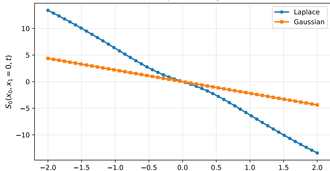
K=1: Score component along x_0 , t = 0.5
