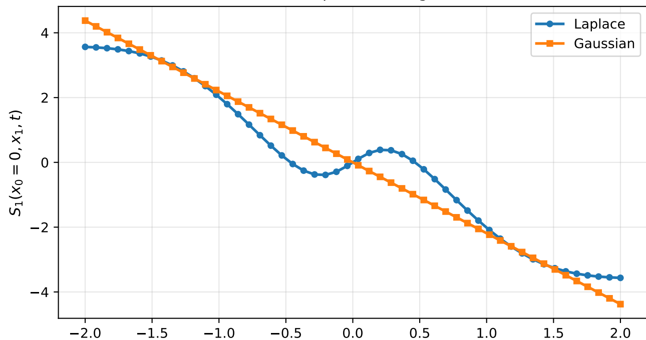
K=1: Score component along x_1 , t = 0.5
