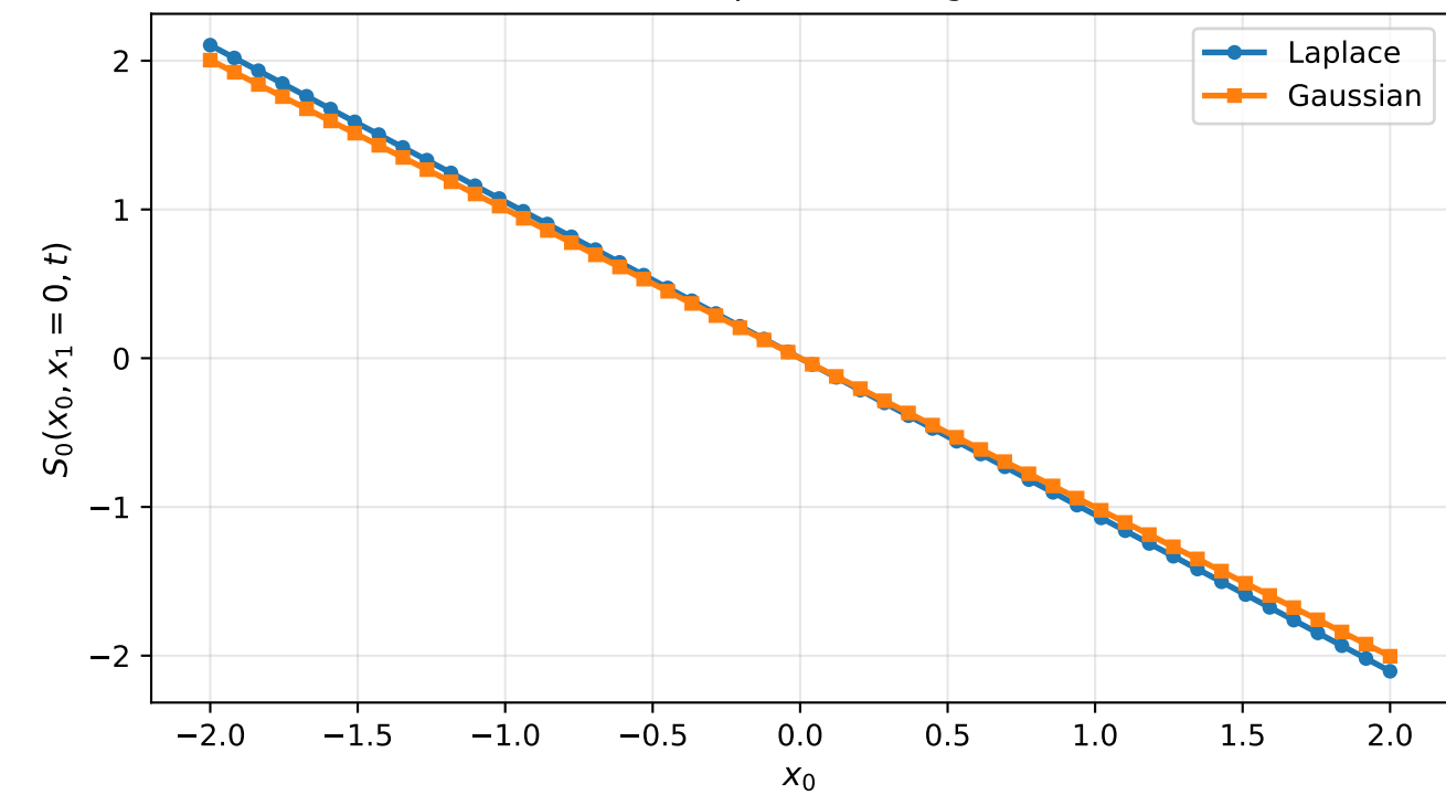
K=1: Score component along x_0 , t = 1.5
