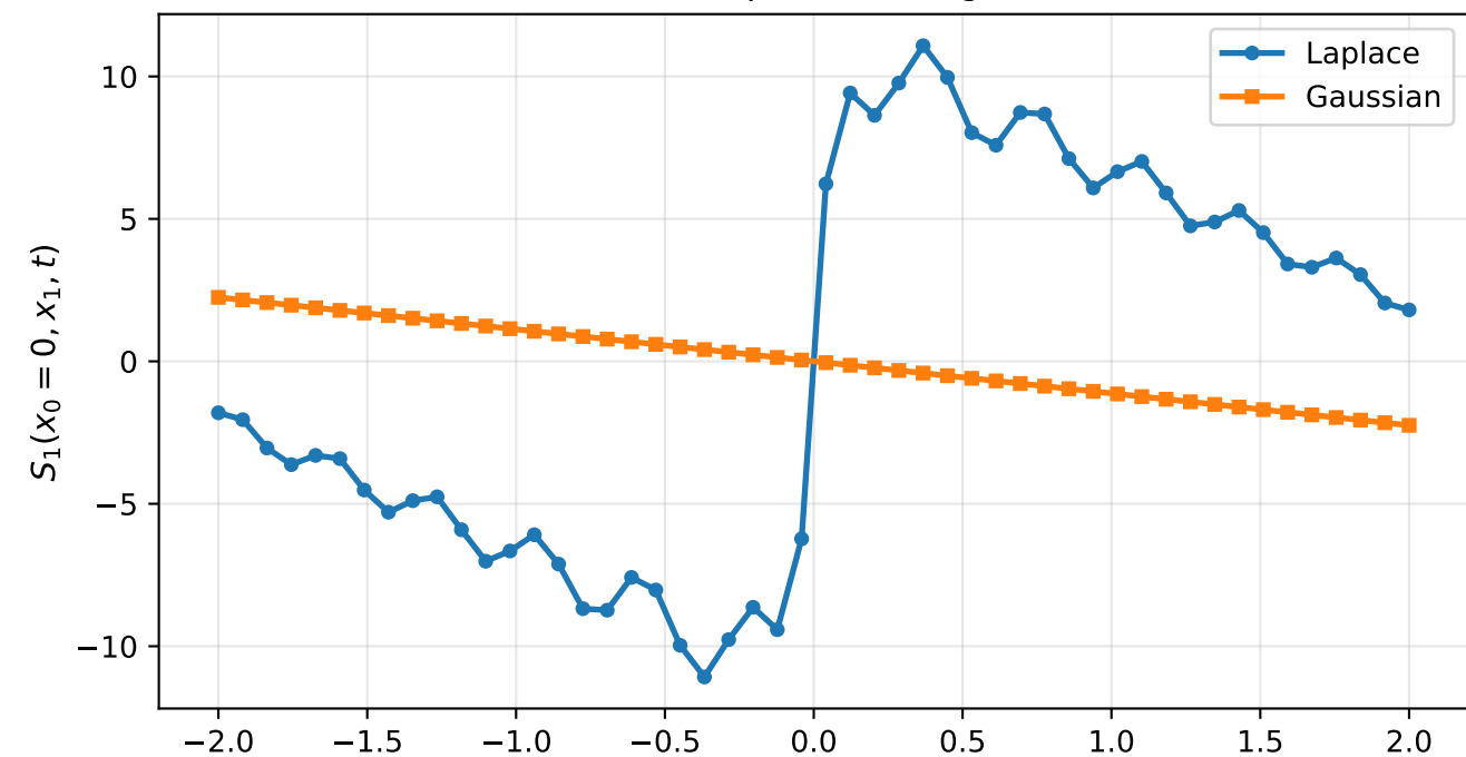
K=1: Score component along x_1 , t = 1.5
