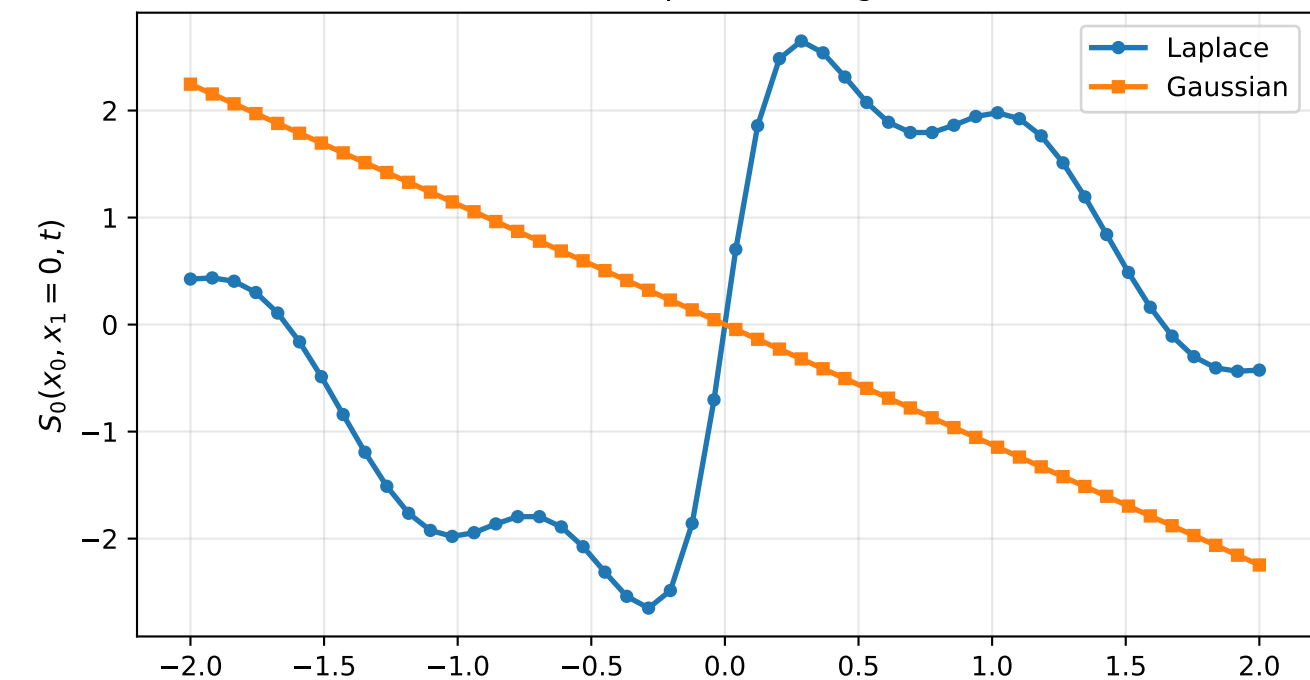
K=1: Score component along x_0 , t = 1.5
