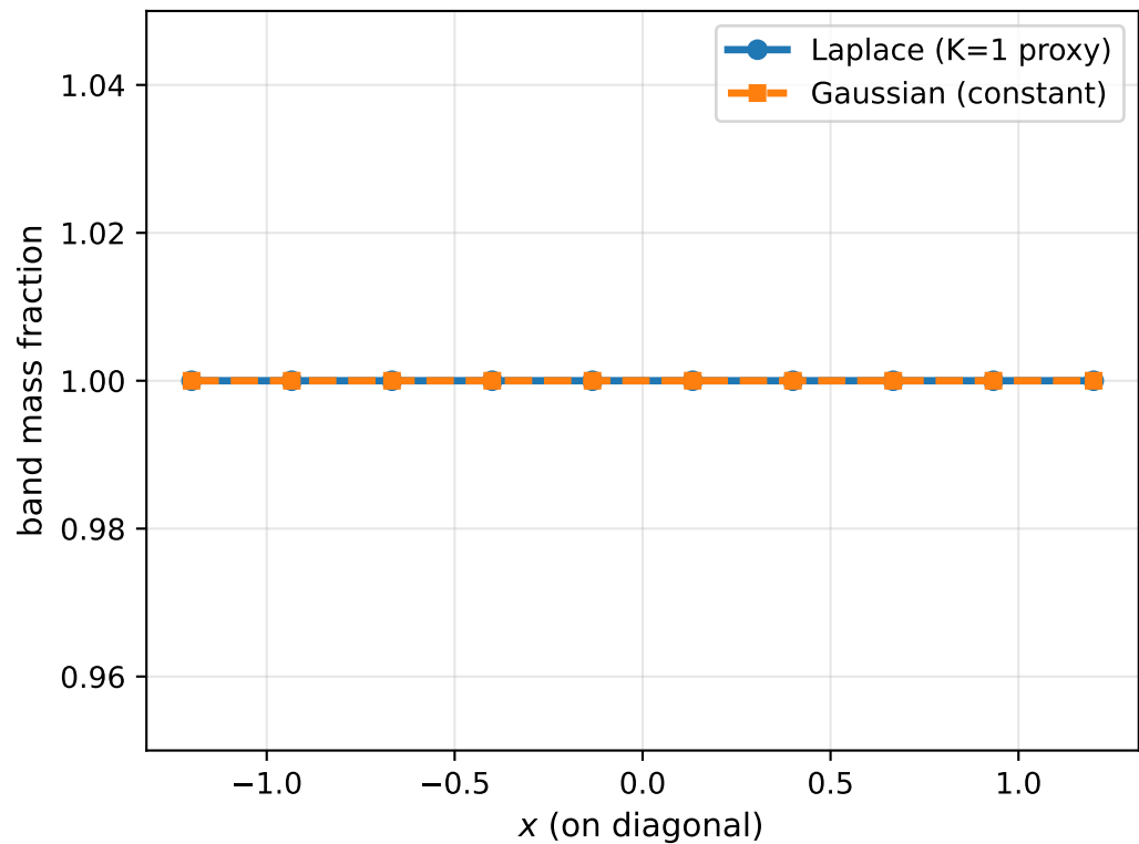
K=2: Hessian tridiagonal mass (K=1 proxy), t = 0.8
