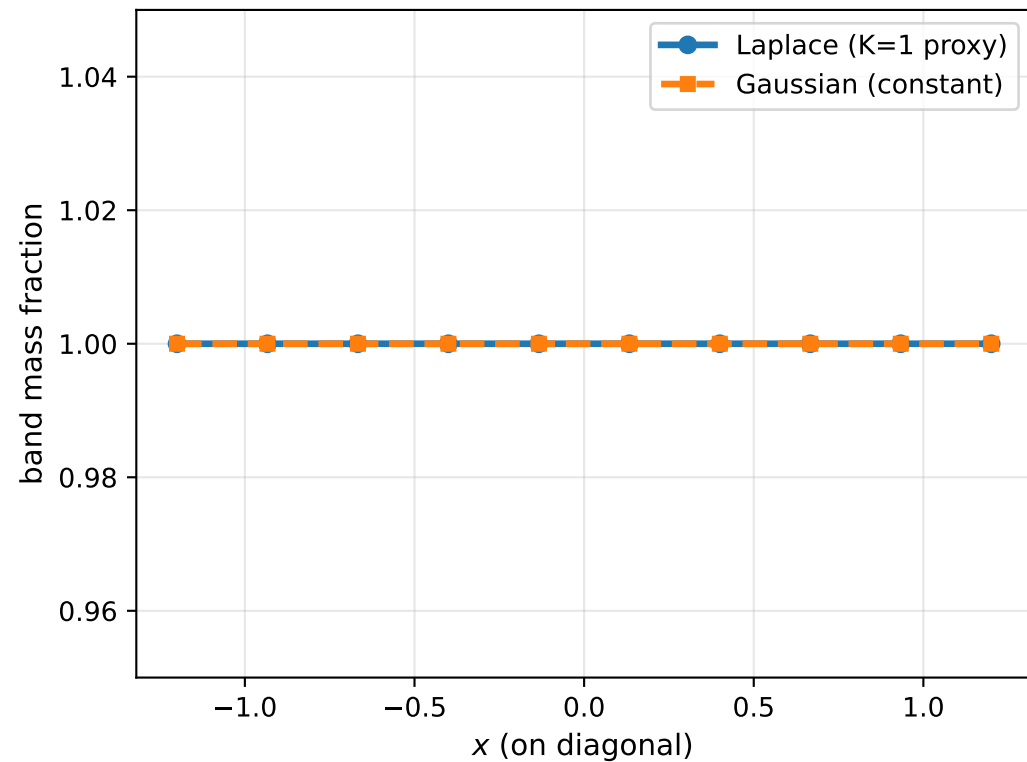
K=2: Hessian tridiagonal mass (K=1 proxy), t = 0.3
