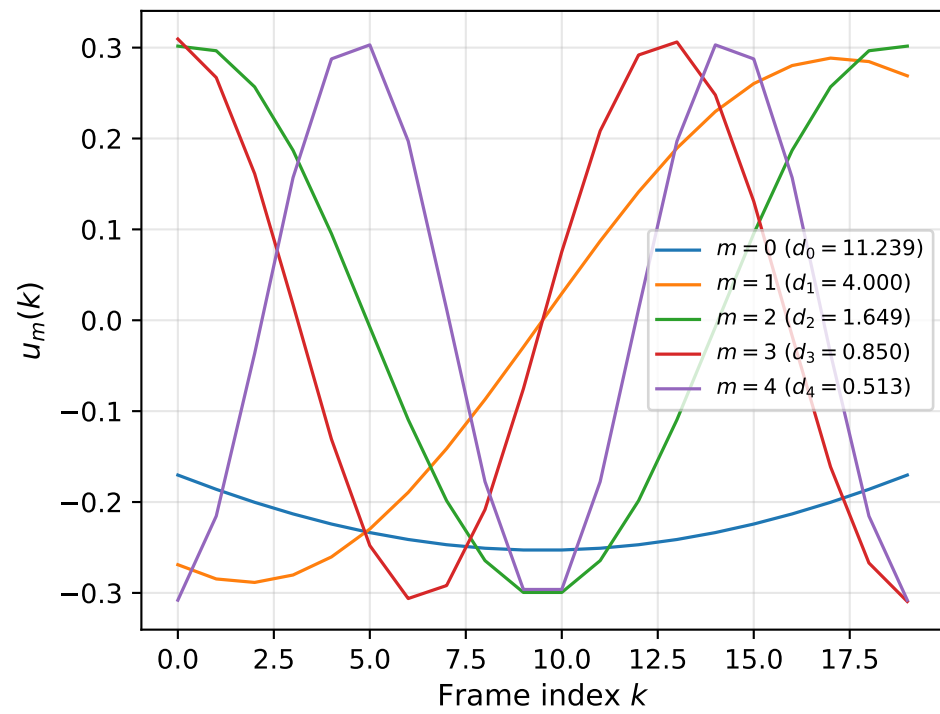
First 5 eigenvectors of \Sigma_0 (shared by all \Sigma_t )
