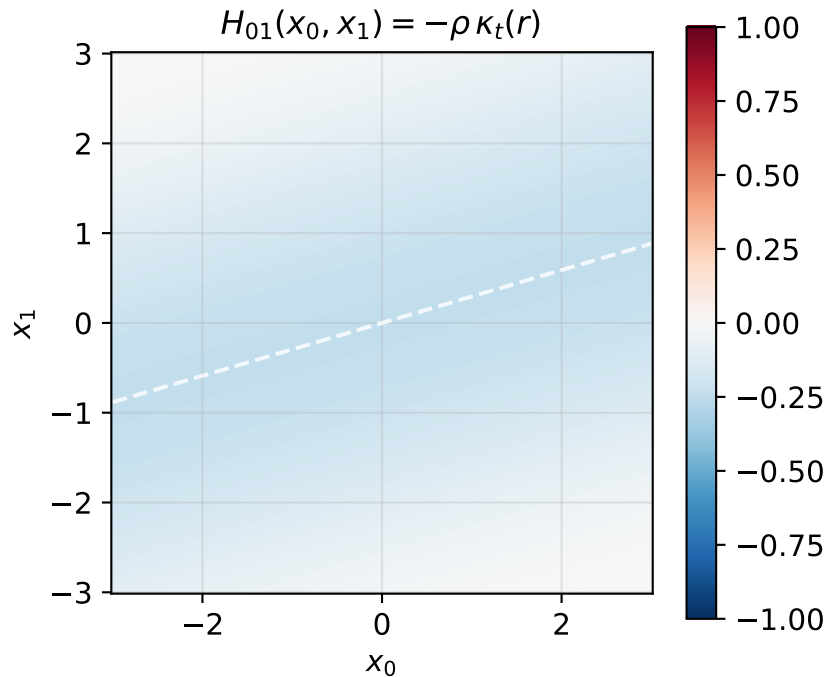
Two-dimensional curvature field with residual ray r = 0 overlaid
