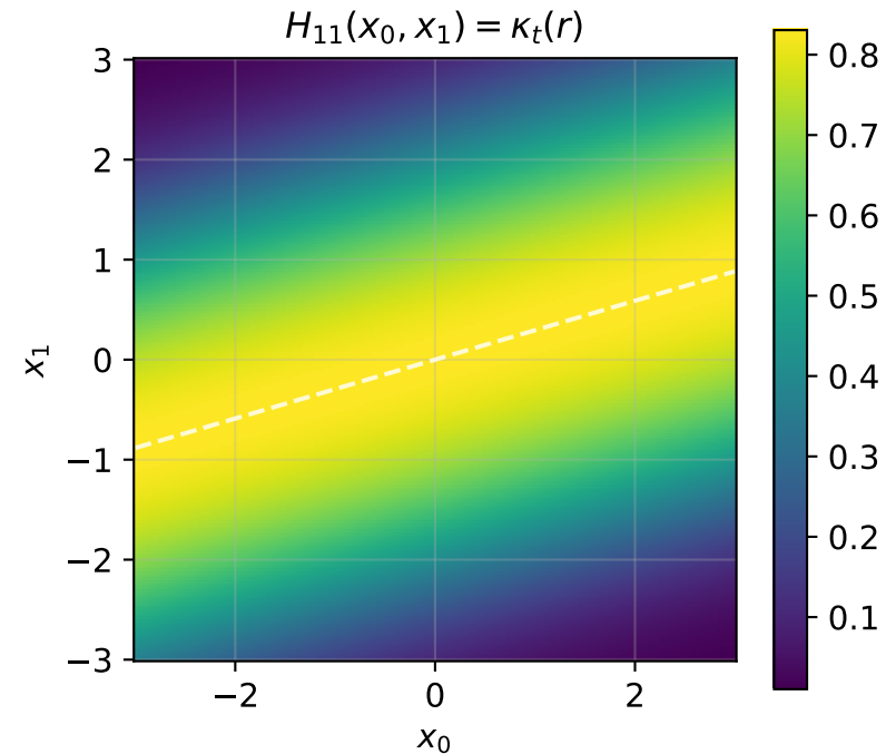
Two-dimensional curvature field with residual ray r = 0 overlaid
