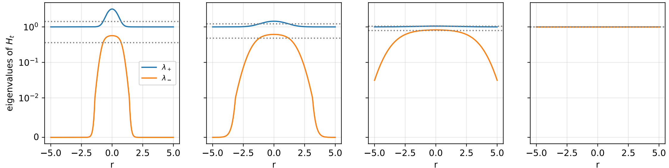
Eigenvalues of the curvature field along the residual ray (dotted: Gaussian benchmark Q_t eigenvalues) t=0.05 t=0.3 t=1.0 t=3.0
