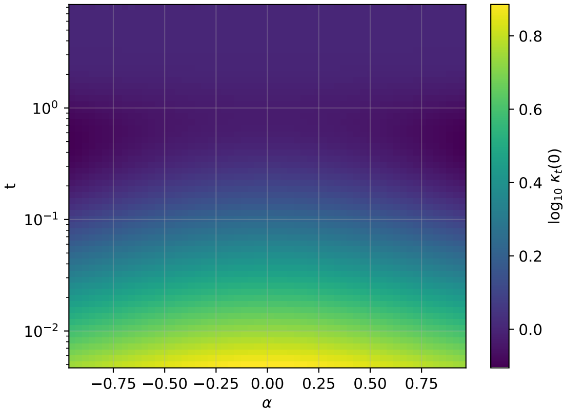
\log_{10} \kappa_t(0) : phase portrait in (\alpha, t)
