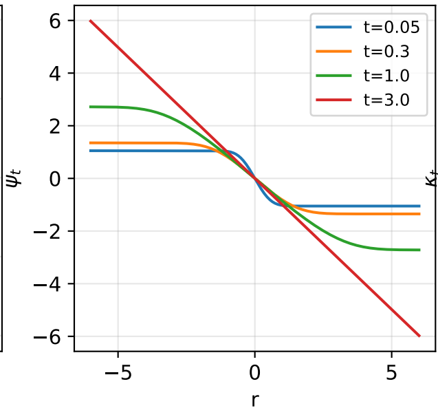
\psi_t(r) = (\log h_t)'(r) residual score
