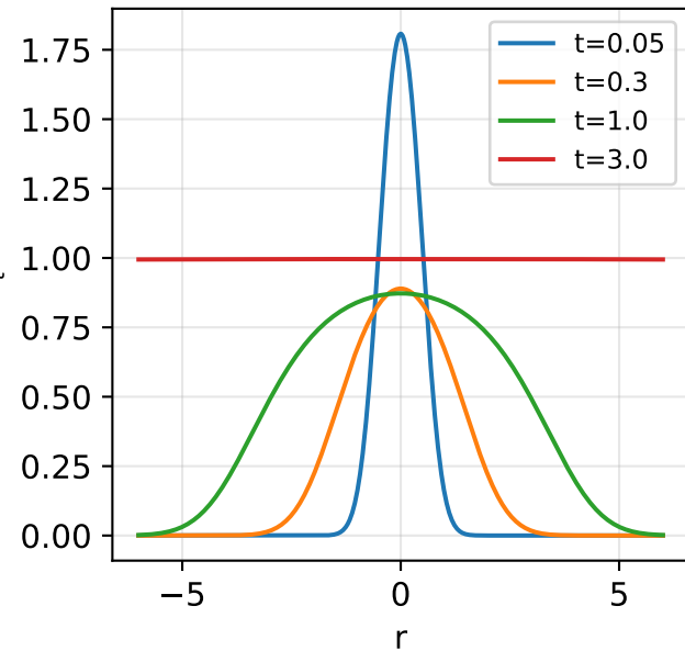
\kappa_t(r) = -(\log h_t)''(r) residual curvature
