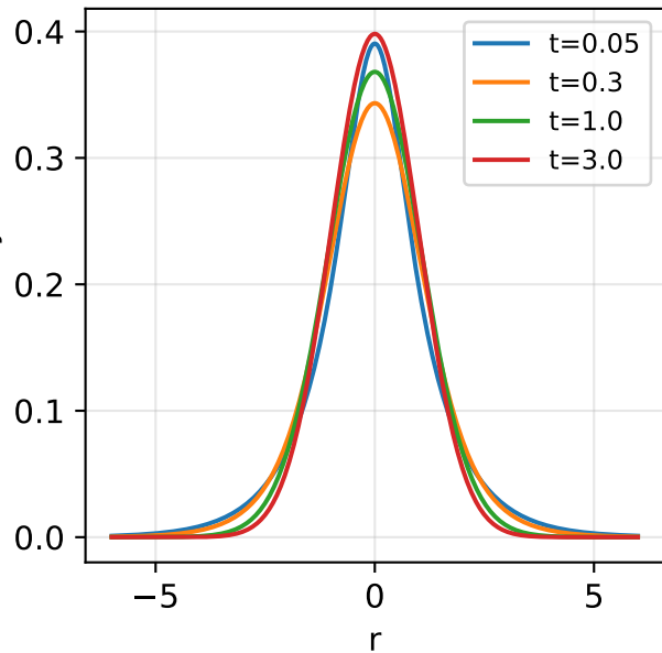
h_t(r) residual density
