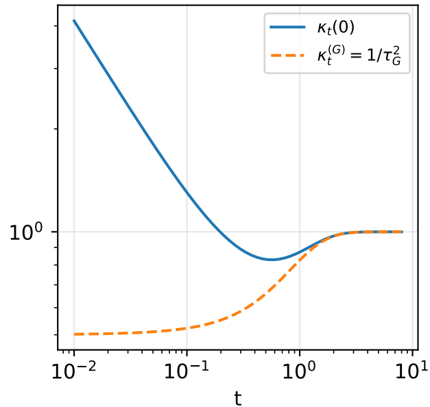
Center vs Gaussian curvature
