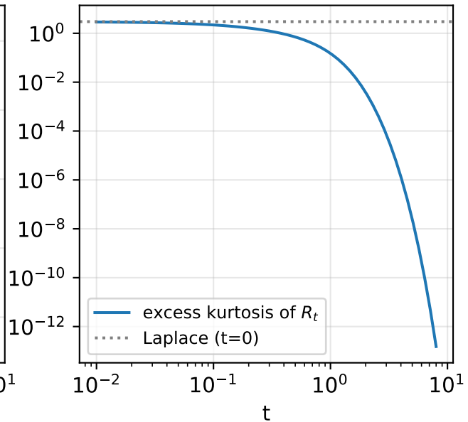
Non-Gaussianity persistence
