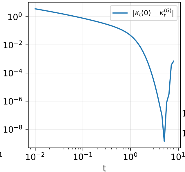
Center-benchmark gap
