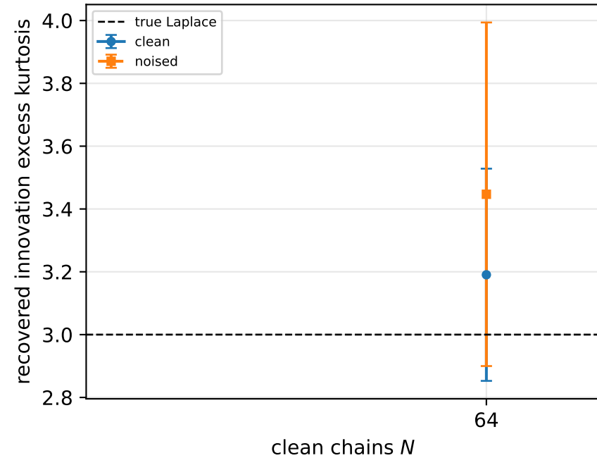
(c) shape: paired gap -0.26 \pm 0.30 ( 0.9\sigma )
