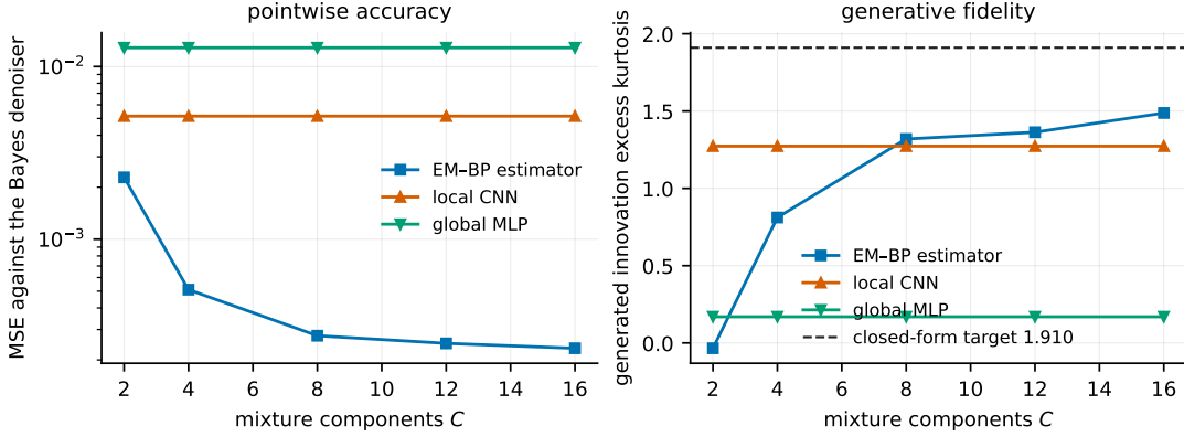
Figure 11.1: Both evaluation axes against the mixture component count. Left: MSE against the Bayes denoiser. Right: generated innovation excess kurtosis against the closed-form target. Both improve monotonically, so the curve moves towards better on both coordinates rather than tracing a trade-off. The network arms are C -independent by construction.
