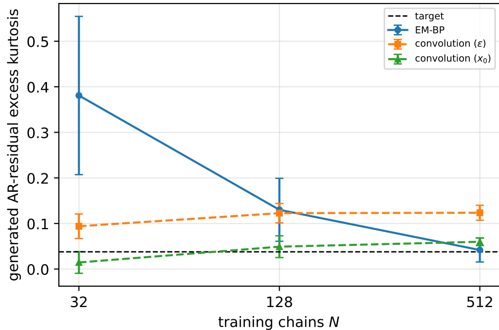
(b) gaussian control -- spread 6.7\times smaller
