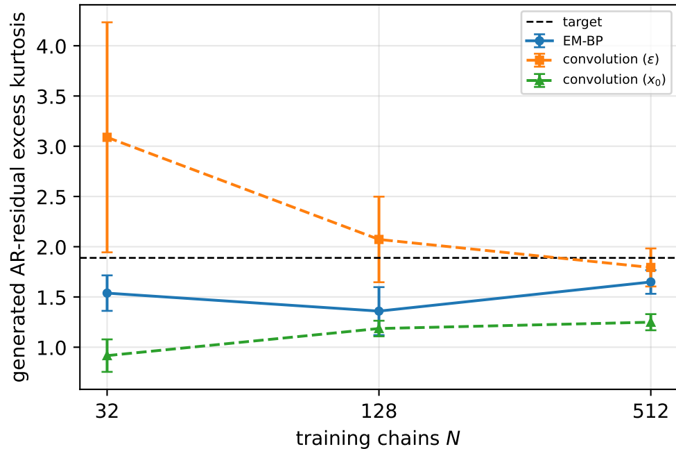
(a) laplace chain -- arms differ by 0.54
