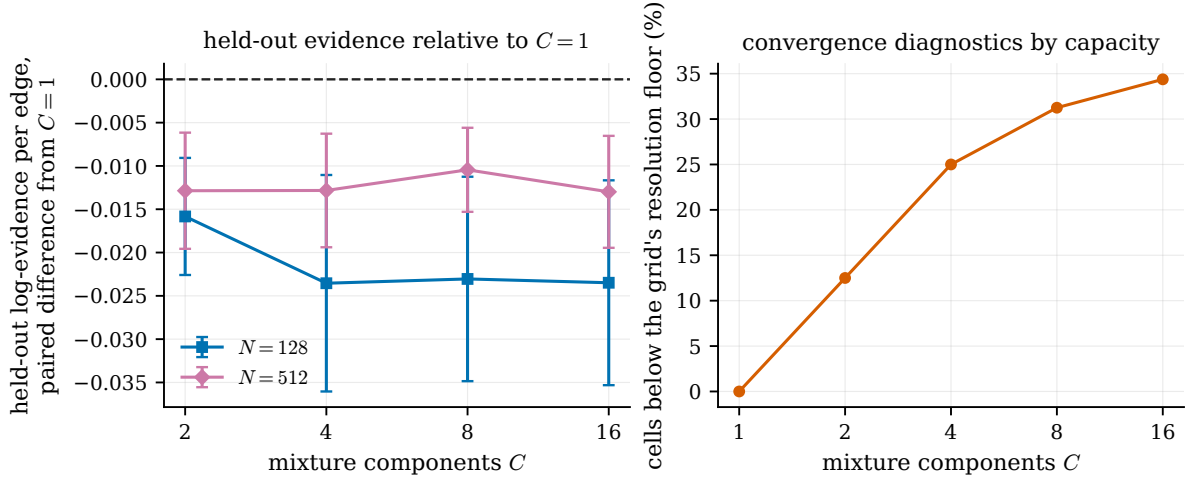
Figure 8.4: Left: the paired difference in held-out log-evidence per edge against C=1 , with one standard error over the 16 seeds. Every interval lies below zero at both training sizes, which is the result of this section. Right: the share of fits whose narrowest component falls under the grid's resolution floor of 2 spacings, which climbs monotonically with C — the second caveat of Remark 8.1, and the reason the left panel is a statement about this estimator on this grid. Every cell at C \geq 4 reached the 1200-iteration cap rather than the convergence tolerance. Both panels are drawn from the cells of Table 8.4.
