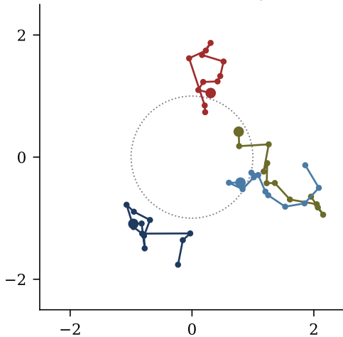
gauged frame: U_\psi a
