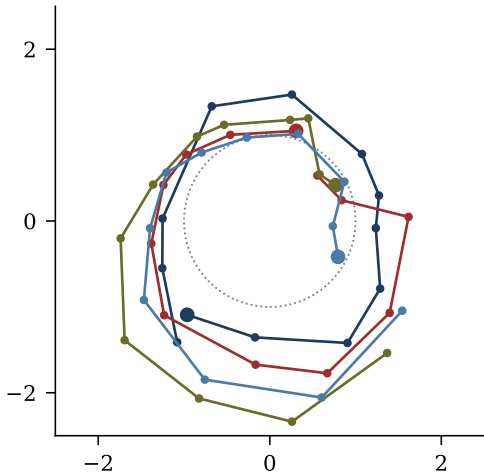
rotating frame: a
