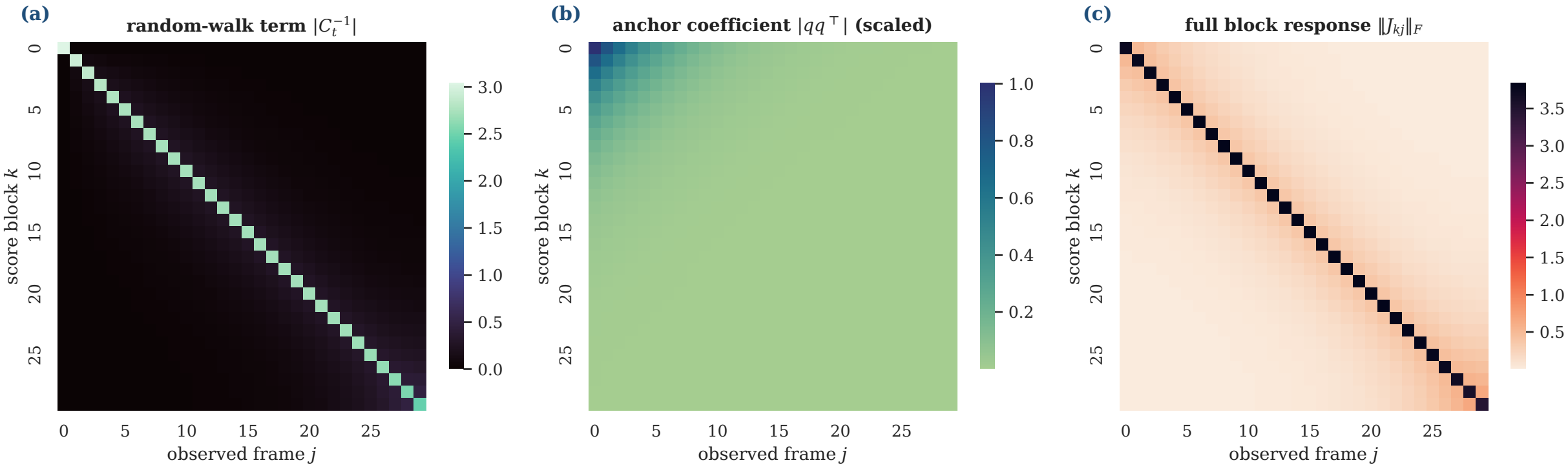
Exact surrogate response at t = 0.20 : near-diagonal chain term plus a rank-one anchor term
