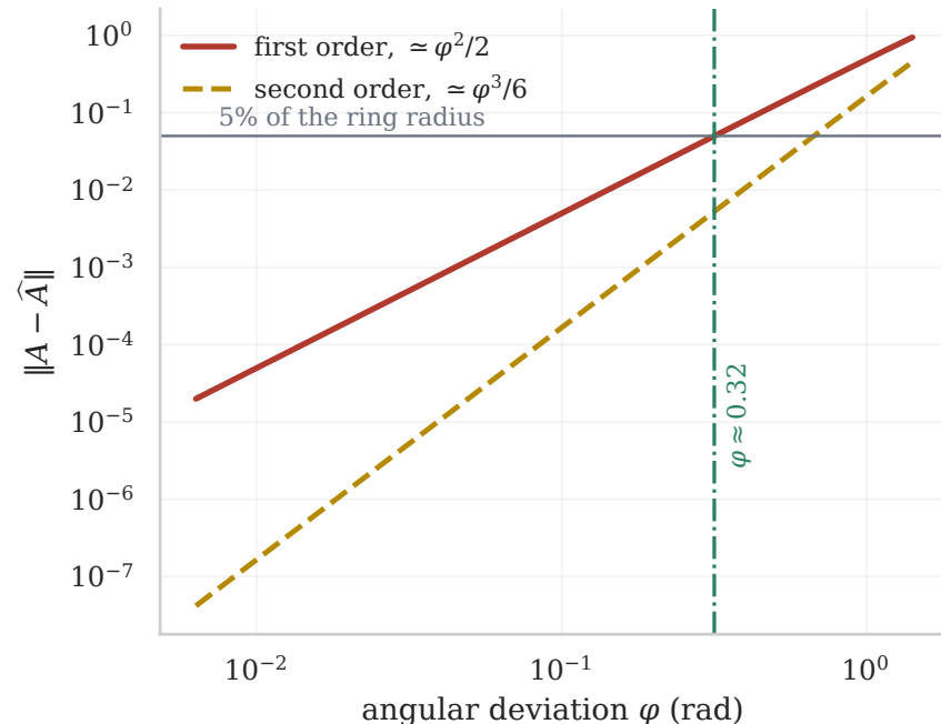
(b) Truncation error of the linearisation
