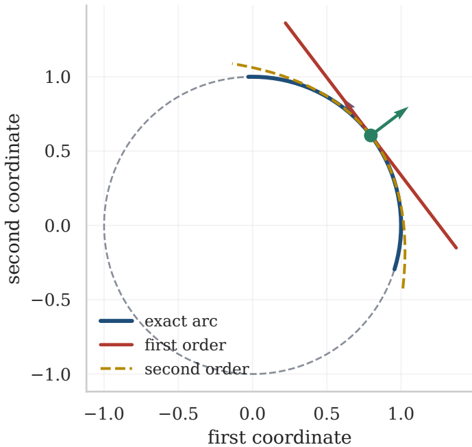
(a) Expanding around one rotating branch
