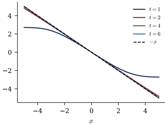
t \rightarrow \infty : Gaussian attractor
