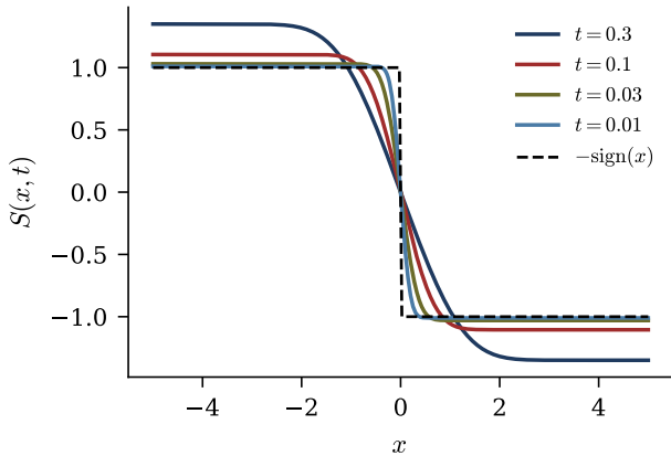
t \rightarrow 0 : prior score
