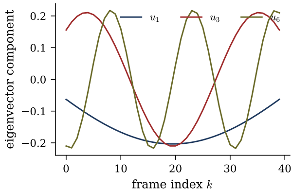
top eigenvectors of \Sigma_0 (near-Fourier)
