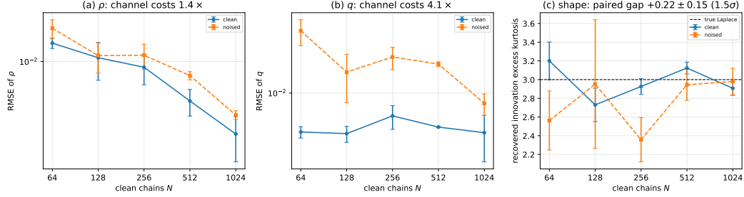
Figure 4: Fitting from clean chains against fitting through the channel, paired: both arms get the same M clean chains and the same 120 iterations, and differ only in whether the chains are observed clean or once each through the OU channel at one of five noise levels. Left, centre: RMSE of \rho and q for the Gaussian kernel, with bootstrap standard errors. Note the clean arm’s q error is flat in M — a discretisation floor, which is why the centre panel’s ratio should be read as indicative. Right: recovered innovation excess kurtosis for the C = 8 mixture on a Laplace chain, where the paired gap is +0.22 \pm 0.15 and therefore not resolved. Three replicates. Source outputs/exp_06_em_parameter_recovery/clean_vs_noised_*.csv.
