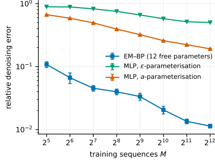
Figure 6: Relative denoising error against training-set size, mean over six replicates with standard errors. The two network curves are the two denoising-score-matching parameterisations reported separately rather than oracle-combined, so the gap to the estimator is visible without the post-selection of Table 1. The fitted innovation density itself is Figure 8 in Appendix I. Source outputs/replicates/merged_summary.csv. Empirical, six replicates.
