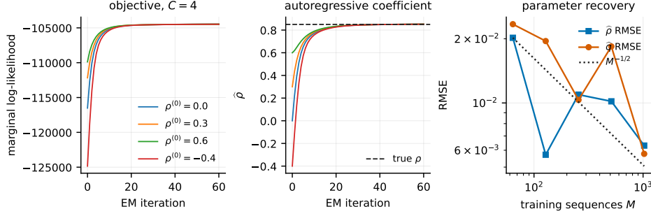
Figure 5: Optimisation diagnostics. Left: marginal log-likelihood by iteration at C = 4 , M = 512 , from four initialisations of \rho ; the largest decrease across iterations is zero in all four, and in the four C = 8 runs not shown. Centre: the estimated autoregressive coefficient over the same runs, converging to [0.8497, 0.8507] against a truth of 0.85 from initialisations spanning [-0.4, 0.6] — direct evidence that \rho is estimated and not supplied. Right: RMSE of the recovered \rho and innovation variance against the number of training sequences, with an M^{-1/2} reference. Sources: outputs/exp_18/em_trace.csv and outputs/exp_06_em_parameter_recovery/em_rate.csv .
