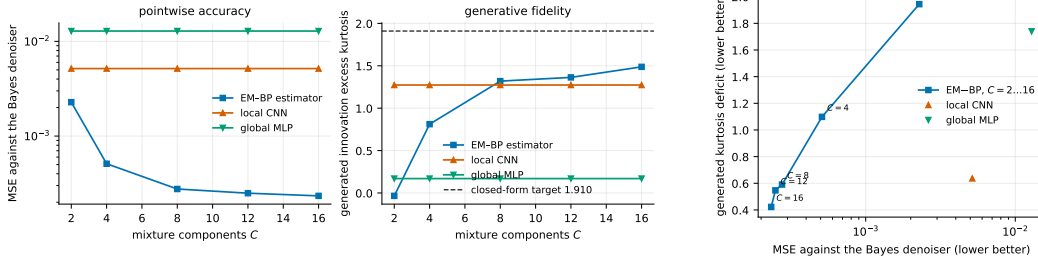
Figure 7: The capacity sweep on both axes. Left and centre: MSE against the Bayes denoiser (log scale) and generated innovation excess kurtosis against the closed-form target, both against C ; the network arms are C -independent by construction. Right: the same data with one axis against the other, one point per configuration — both coordinates improve together, so the trace moves towards the origin rather than along a trade-off. Data as in Table 2. Empirical, three seeds; the sweep does not yet include marginal likelihood or runtime against C .
