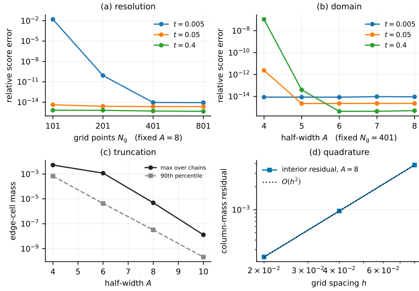
Figure 8.1: Grid and domain control on a Laplace chain ( \alpha = 0.85 , n = 32 sites). Left: relative score error against a high-resolution reference as grid resolution M grows at fixed half-width A = 8 . Right: the same as the domain half-width A grows at fixed M = 401 . Both saturate at the floating-point floor well inside the working configuration. Source: outputs/exp_02_grid_convergence/ .
