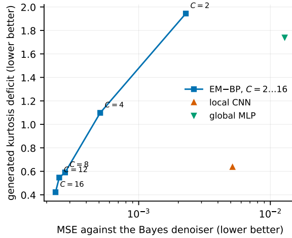
Figure 9.3: Pointwise denoising MSE against generated-sample excess kurtosis, one point per estimator/capacity configuration. The two axes are not a trade-off curve for a single estimator; the sharper statement is the within-arm MLP result reported in the text. Source: outputs/exp_16/gen2_n*/ .
