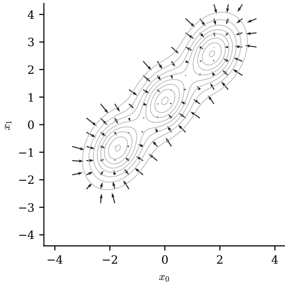
joint score field \nabla \log p_t
