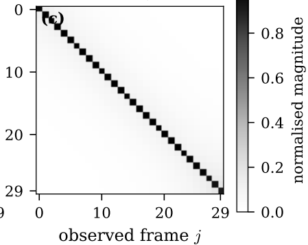
full \|J_{kj}\|_F
