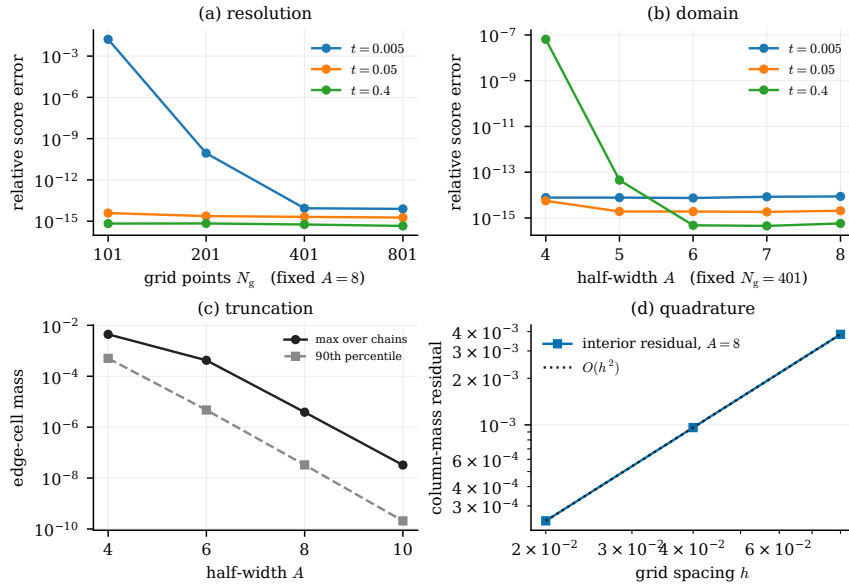
Figure 8.1: Grid and domain control on a Laplace chain ( \alpha = 0.85 , L = 32 sites), four panels. (a) Relative score error against a high-resolution reference as grid resolution N_g grows at fixed half-width A = 8 ; (b) the same as A grows at fixed N_g = 401 — both saturate at the floating-point floor well inside the working configuration. (c) Forward-message boundary mass against A , the truncation diagnostic, drawn as both the maximum and the 90th percentile over 256 chains, which differ by roughly two orders of magnitude for the reason given in Remark 8.4. (d) Interior column-mass residual against spacing at A = 8 , the quadrature diagnostic, with an O(h^2) reference. Neither diagnostic alone certifies convergence. Source: outputs/frozen/exp_01/ and outputs/frozen/exp_18/ .
