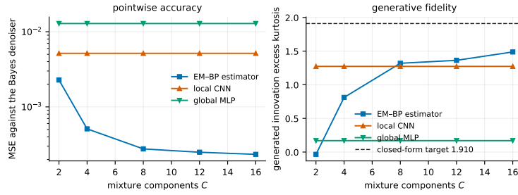
Figure 11.2: Held-out denoising MSE and generated-sample fidelity against mixture capacity C , three seeds, at a fixed EM budget of 40 iterations. Read alongside the caveat below: the shape-dependent curves in this figure are confounded with EM convergence rate; the evidence-based saturation reported in the text, from a separate paired design, is not. Source: outputs/exp_16/ .
