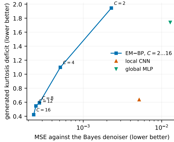
Figure 11.3: Pointwise denoising MSE against generated-sample excess kurtosis, one point per estimator/capacity configuration. The two axes are not a trade-off curve for a single estimator; the sharper statement is the within-arm MLP result reported in the text. Source: outputs/exp_16/gen2_n*/ .
