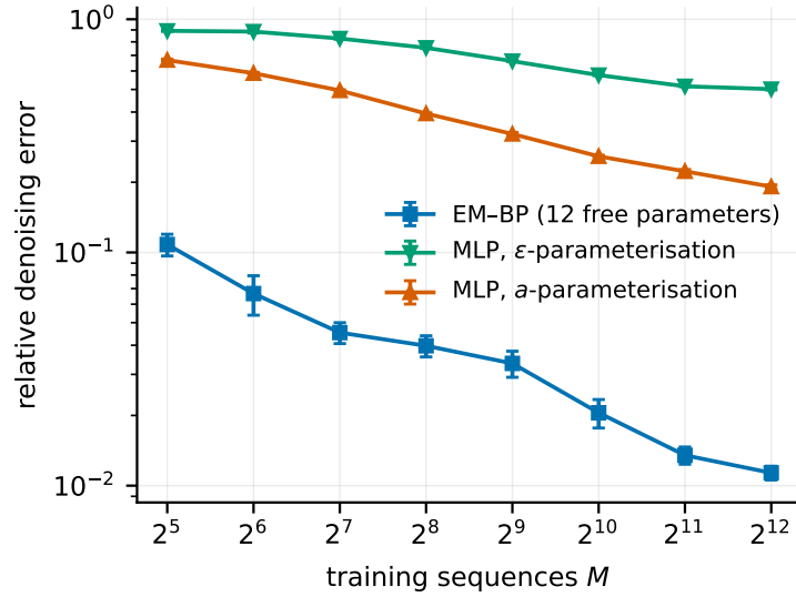
Figure 11.1: Relative denoising error against training-set size, mean over six replicates with standard errors, for the EM/BP estimator and the two network baselines reported separately. Source: outputs/exp_07_em_vs_score_network/ .
