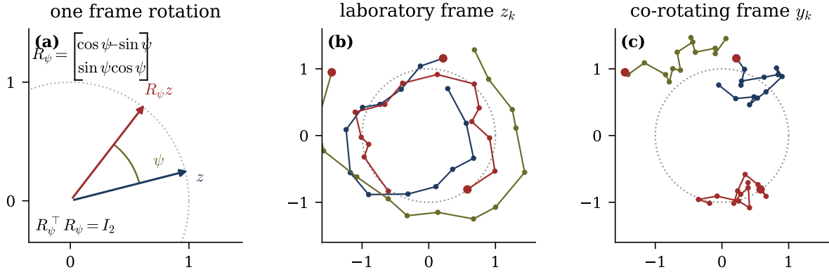
Figure 7.2: The rotation and the gauge. (a) R_\psi turns every vector through the same angle without changing its length, which is the statement R_\psi^T R_\psi = I_2 . (b) Three surrogate trajectories in the laboratory frame ( K = 14 , \sigma = 0.16 , \psi = 2\pi/14 ; the marked point is k = 0 ), coherently circulating. (c) The same trajectories after U_\psi : a random walk anchored on the ring. Because U_\psi is orthogonal the reduction is exact at every diffusion time; the numerical round trip agrees to machine precision (Table 7.1).
