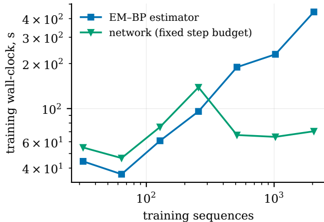
training cost
