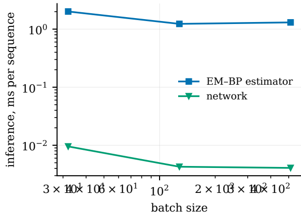
inference cost
