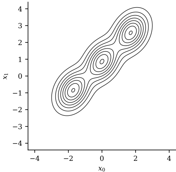
noised joint density p_t(x_0, x_1)
