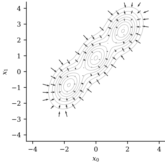
joint score field \nabla \log p_t
