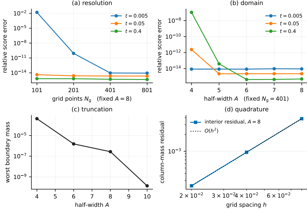
Figure 9.1: The two error sources, measured separately. (a) Relative score error against the number of grid points at fixed A = 8 , and (b) against the half-width at fixed N_g = 401 ; both saturate at the floating-point floor \sim 10^{-14} , beyond which the curves measure arithmetic rather than discretisation. (c) Worst boundary mass over 32 sites against A : the truncation diagnostic, near-independent of N_g . (d) Interior column-mass residual of the transition matrix against spacing at A = 8 : the quadrature diagnostic, following O(h^2) as the trapezoidal rule predicts. Panels (a)–(b) from outputs/exp_01_grid_validation/grid_heatmap.csv , (c)–(d) from outputs/exp_18/boundary.csv .
