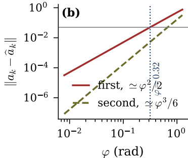
truncation error
