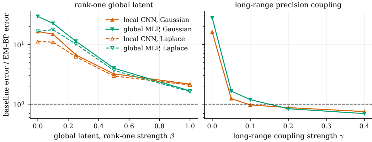
Figure 8.5: The same cells as Table 8.5, on a logarithmic vertical axis with the break-even line drawn; solid is the Gaussian innovation, dashed with open markers the Laplace one. The two mechanisms are not two amounts of the same thing: under a rank-one global latent the advantage decays smoothly and does not reach the line, even where half the marginal variance is a shared constant; under long-range coupling it crosses within the first tested strength and stays below. The Laplace curves track the Gaussian ones across the whole rank-one sweep, which shows that the rank-one result is not confined to the Gaussian experiment; its generality beyond these two innovation families remains open. The long-range panel is Gaussian only, since the contaminated Laplace model has no closed-form reference. Every curve is a mean over the noise schedule, so it shows the direction rather than the worst case — the tie reported in the text at \beta = 1 is at one noise level and is not visible here. All fall because the estimator degrades, not because the baselines improve: the last row of each block in Table 8.5 carries EM-BP’s own error.
