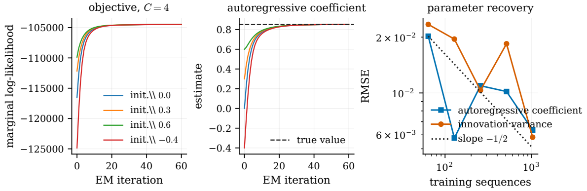
Figure 7.2: Optimisation diagnostics for the EM procedure of Section 7.3. Left: marginal log-likelihood by iteration from four initialisations of \alpha ; the largest decrease across iterations is zero in every run. Centre: the estimated \alpha over the same runs, converging to [0.8517, 0.8520] against a truth of 0.85 from initialisations spanning [-0.4, 0.6] — direct evidence that \alpha is estimated, not supplied. Right: RMSE of the recovered \alpha and innovation variance against the number of training sequences, with an n^{-1/2} reference line. Source: outputs/exp_18/ and outputs/exp_06_em_parameter_recovery/ .
