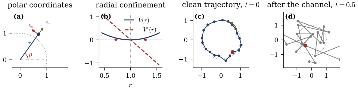
Figure 9.1: The rotating-ring model, at the parameters used throughout this chapter ( L = 20 , \kappa = 2 , D_r = 0.015 , D_\theta = 0.005 , \omega = 1 , h = 2\pi/20 ). (a) Polar coordinates and the moving frame (9.4). (b) The potential (9.5) and the force (9.6) it generates; the force changes sign at r = 1 , which is therefore the stable radius. (c) One clean trajectory, a noisy coherently turning path near the unit circle; the arrow marks the sense of rotation. (d) The same trajectory after the channel (9.8) at t = 0.5 , from a single standardised noise realisation.
