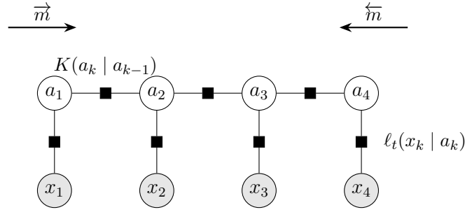
Figure 3.1: The posterior factor graph of a Markov chain observed through the coordinatewise channel. Open circles are latent variables, shaded circles observations, squares factors. Each transition factor K(a_k | a_{k-1}) joins two adjacent latent variables; each observation enters through a unary factor attached to a single latent variable, because the channel corrupts every coordinate independently. Conditioning therefore reweights node potentials without creating any edge among the a_k , so the posterior graph is still a chain and Theorem 3.3 applies to it. Arrows show the two message sweeps of (3.3). The construction fails as soon as the forward noise is correlated across coordinates: the likelihood then touches several a_k at once and the graph acquires edges.
