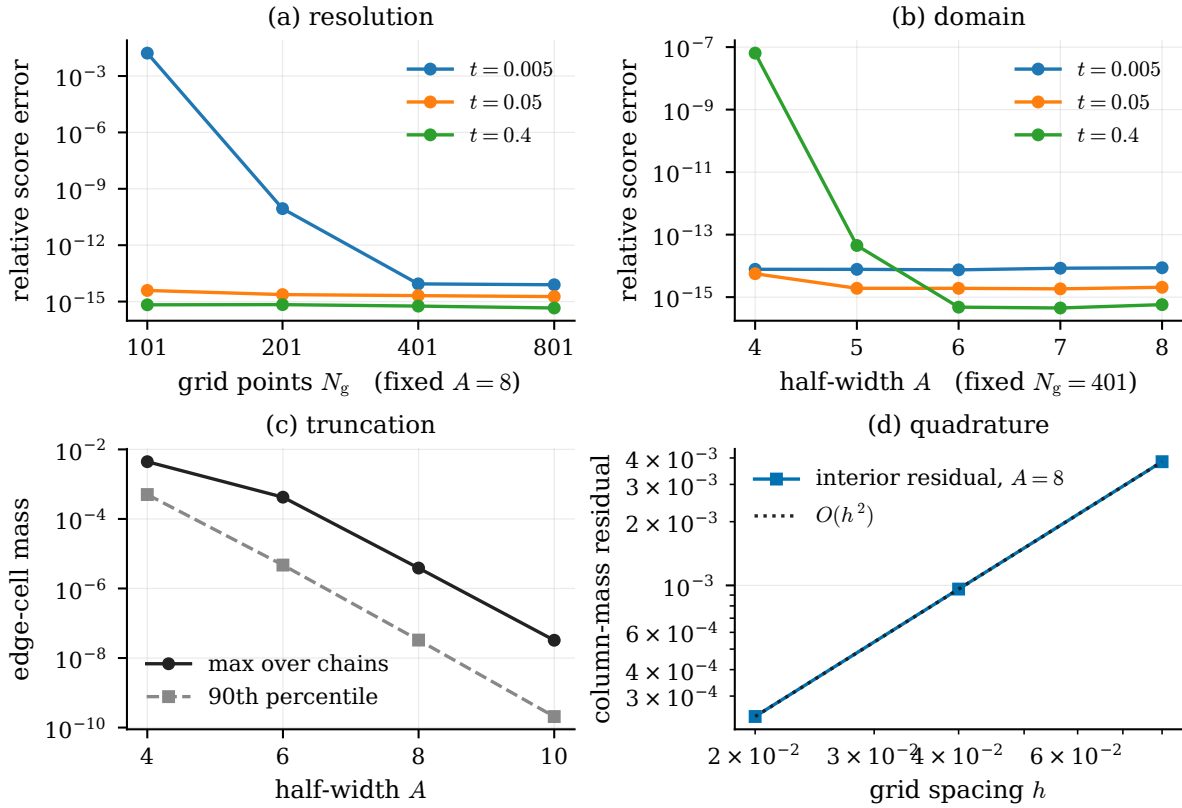
Figure 7.1: Grid and domain control on a Laplace chain ( \alpha = 0.85 , L = 32 sites), four panels. (a) Relative score error against a high-resolution reference as grid resolution N_g grows at fixed half-width A = 8 ; (b) the same as A grows at fixed N_g = 401 — both saturate at the floating-point floor well inside the working configuration. (c) Forward-message boundary mass against A , the truncation diagnostic, drawn as both the maximum and the 90th percentile over 256 chains, which differ by roughly two orders of magnitude for the reason given in Remark 7.4. (d) Interior column-mass residual against spacing at A = 8 , the quadrature diagnostic, with an O(h^2) reference. Neither diagnostic alone certifies convergence. Source: outputs/frozen/exp_01/ and outputs/frozen/exp_18/ .
