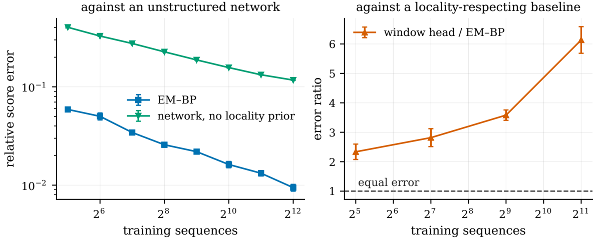
Figure 8.3: The two comparisons together. Left: relative score error against training-set size for EM-BP and a network given no locality prior, with one standard error over the 16 seeds. Right: the paired per-seed ratio of window-head risk to EM-BP risk, against a baseline that does have locality and weight sharing, with the break-even line drawn. The left gap is the headline 7.0–17.6 \times ; the right one is 2.3–6.1 \times , and the difference between the two panels is how much of the headline margin does not survive supplying those two structural biases. Both ratios grow across the tested sizes. That is a description of four measured sizes, not a mechanism: different statistical rates and different optimisation limits produce the same signature, and no design here separates architecture, parameter sharing, capacity and optimisation, which change together when the baseline is swapped. Drawn from the same certified cells as Tables 8.1 and 8.3.
