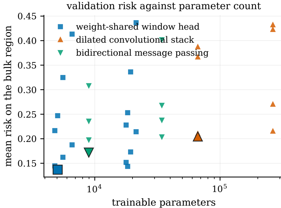
Figure 8.2: Every configuration of the screen, scored on the bulk region and averaged over the 4 development seeds. One marker per architecture; the outlined marker is each architecture’s best configuration. The horizontal axis is what makes the comparison readable: the dilated stack sits an order of magnitude to the right and does not reach the window head’s risk anywhere in the screen. Drawn from the same artifact as Table 8.2.
