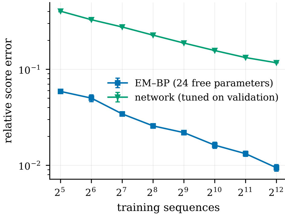
Figure 8.1: Relative score error against training-set size, mean over 16 replicates with standard errors, for the EM-BP estimator and the validation-tuned MLP. The window-head baseline of Section 8.2 scores every site rather than the aggregate plotted here and is reported as a ratio table (Table 8.3) rather than superimposed on this figure. Drawn from the same outputs, over the same size grid and with the same seed-first aggregation, as Table 8.1.
