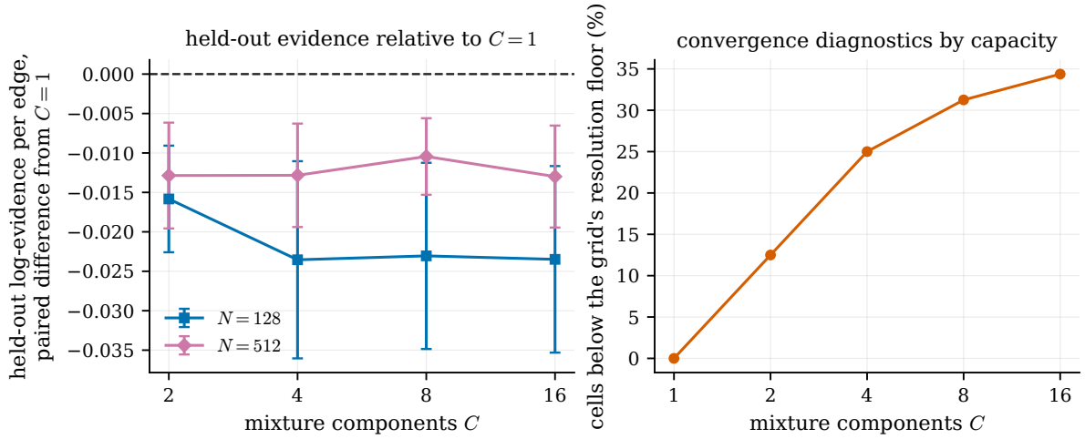
Figure 8.4: Left: the paired difference in held-out log-evidence per edge against C = 1 , with one standard error over the 16 seeds. Every interval lies below zero at both training sizes, which is the result of this section. Right: the share of fits whose narrowest component falls under the grid’s resolution floor of 2 spacings, which climbs monotonically with C — the second caveat of Remark 8.1, and the reason the left panel is a statement about this estimator on this grid. Every cell at C \geq 4 reached the 1200-iteration cap rather than the convergence tolerance. Both panels are drawn from the cells of Table 8.4.
