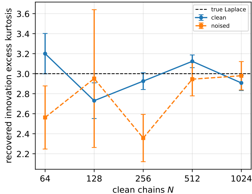
(c) shape: paired gap +0.22 \pm 0.15 (1.5\sigma)
