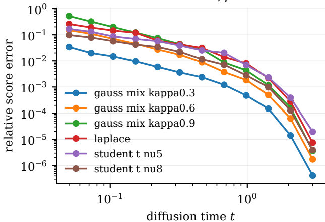
Gaussian baseline, \rho = 0.85
