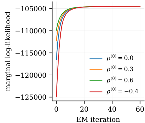
objective, C = 4
