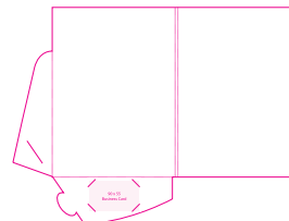
05 Dbl Flap 5mm Gusset
