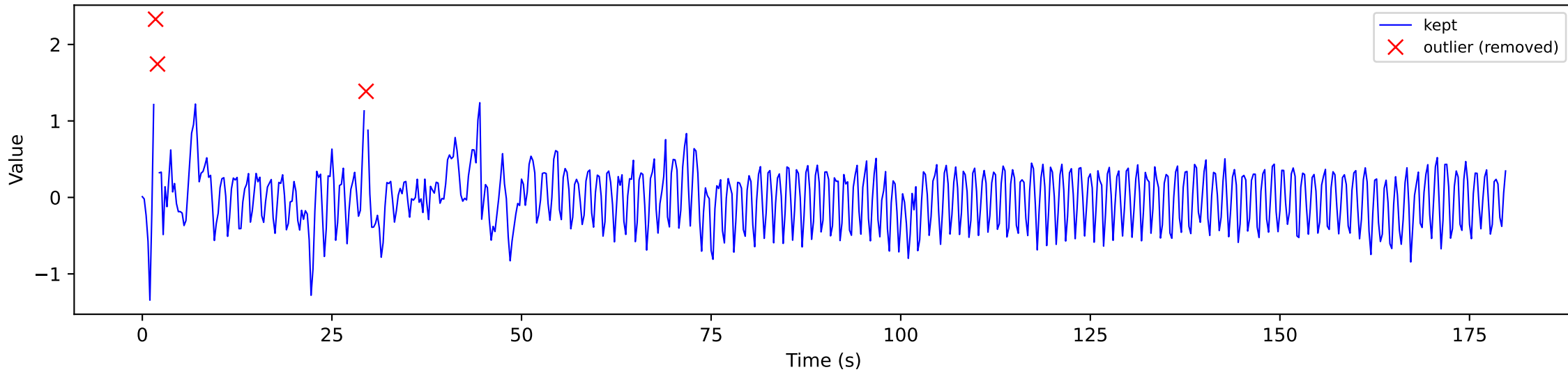
gyr_z — after Chauvenet outlier removal (C=2)
