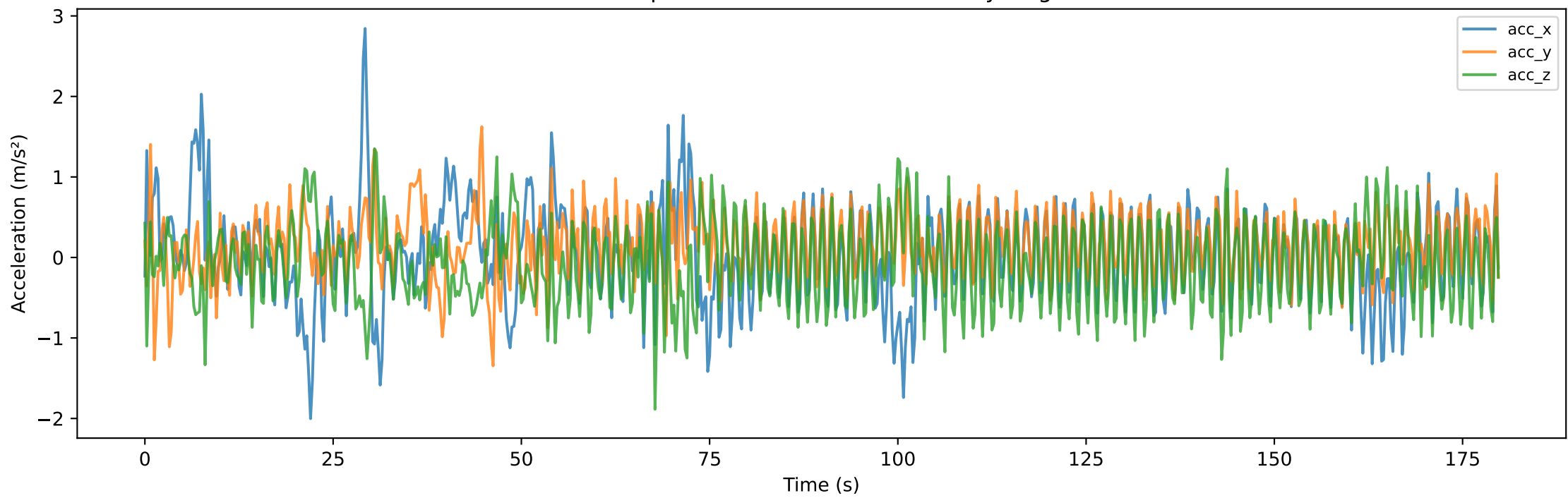
Final processed accelerometer — walking
