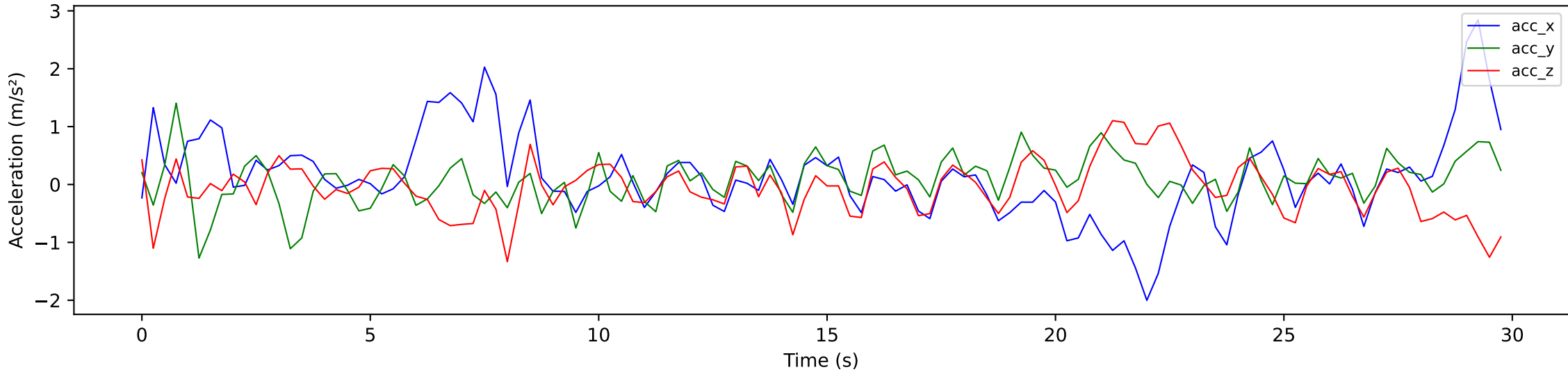
Accelerometer — after low-pass filter (cutoff=1.5 Hz)
